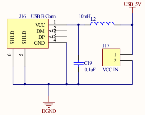
Computer Side Logic Power (5V)
